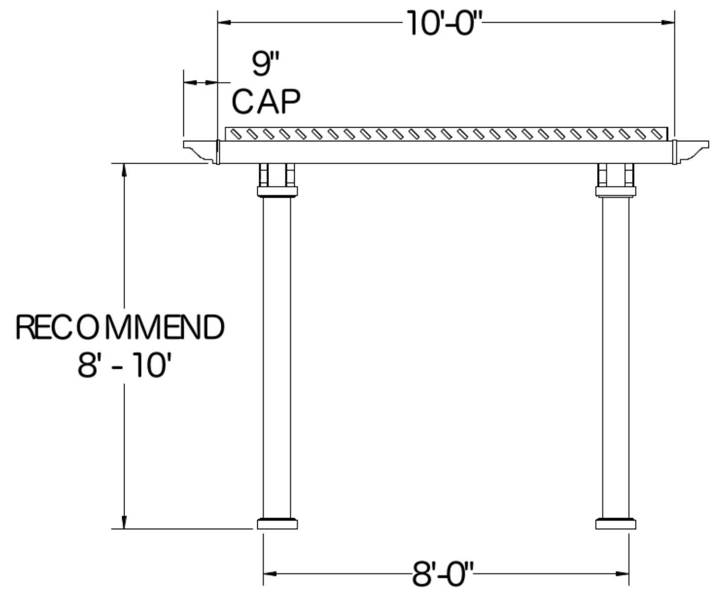
Center of Post to Structure Measurement
