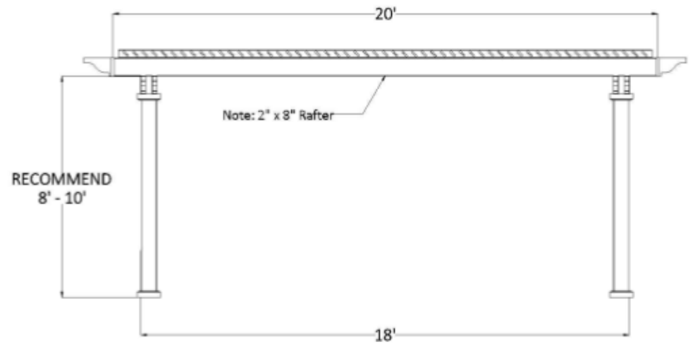
Center of Post to Structure Measurement
