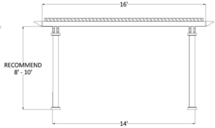
Center of Post to Structure Measurement
