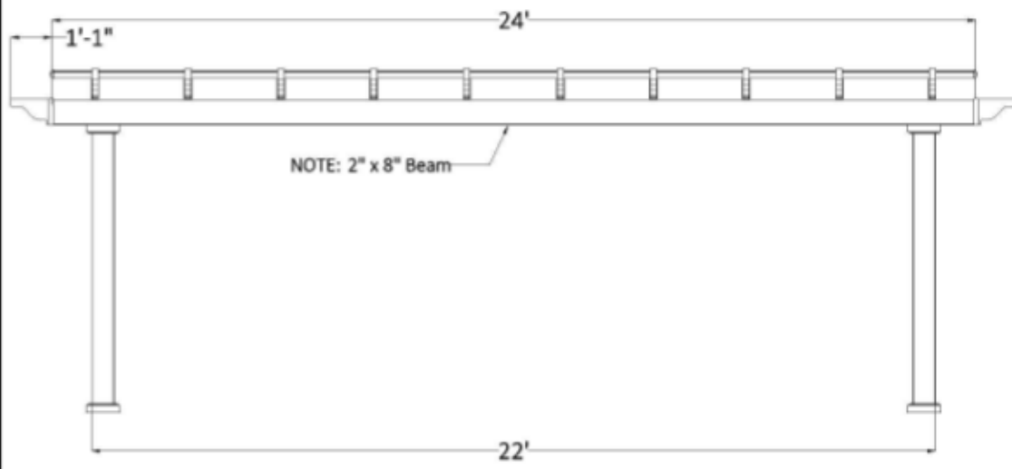
Post on Center Measurement
