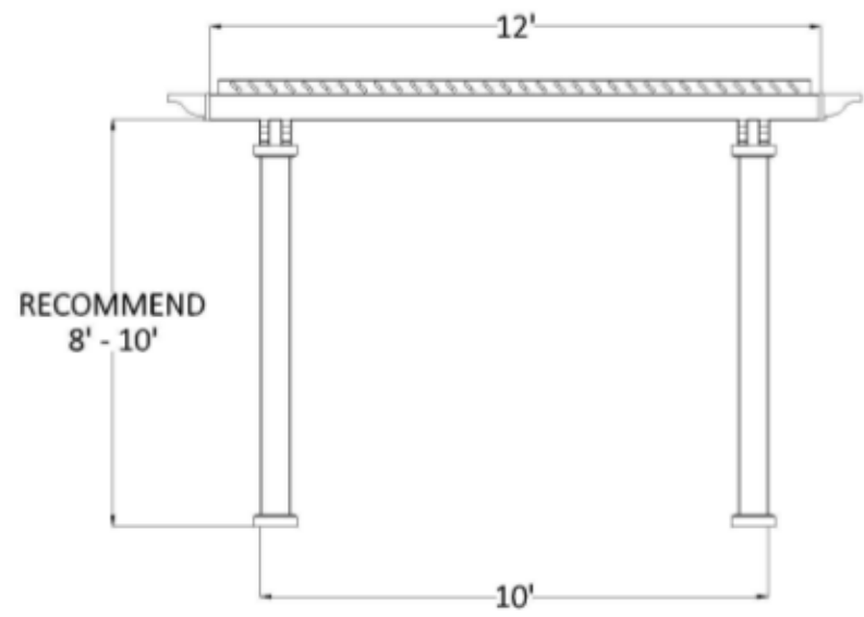
Center of Post to Structure Measurement
