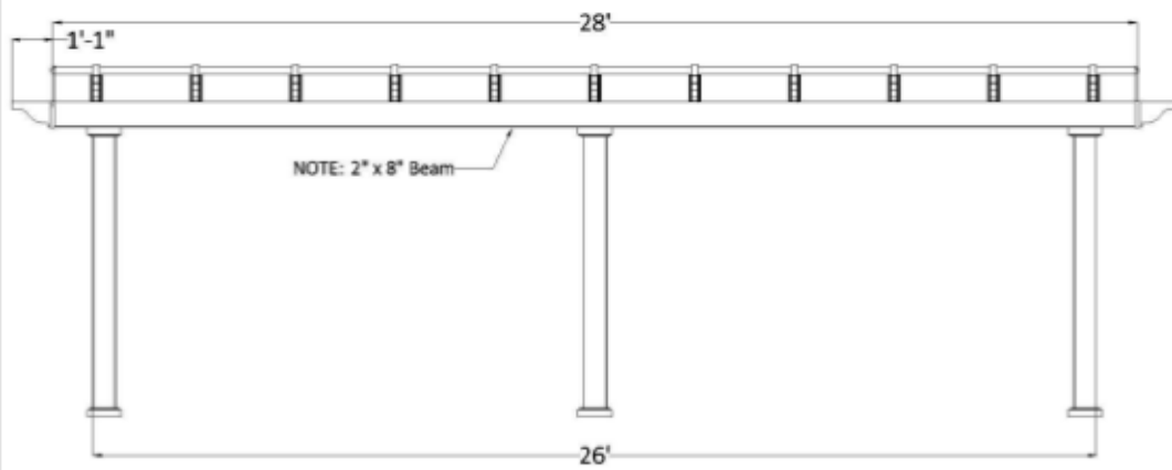
Post on Center Measurement
